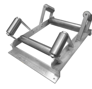
▷ 12" & 15" COIL CRADLES
